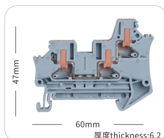
JHPTV-4TW
