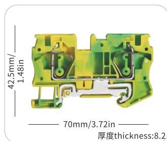
JHST-6PE
