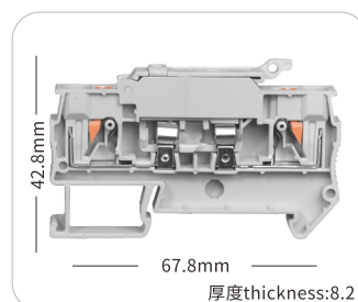
JHPTC-4HESI
