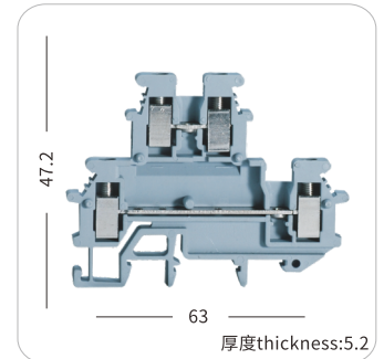
JHUKK 2.5
