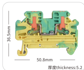
JHPTV-2.5PE
