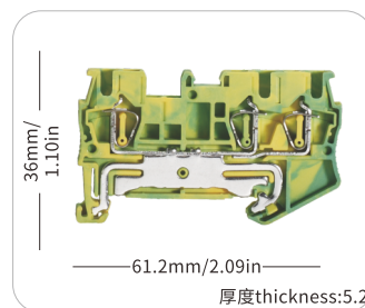
JHST-2.5TWPE
