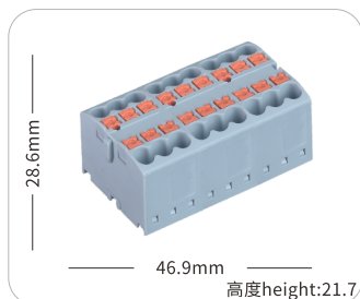
JHPTX-18
