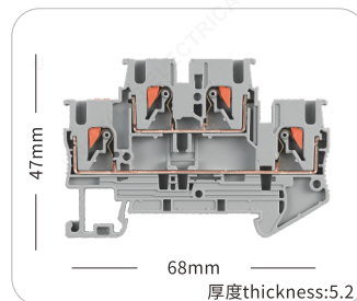
JHPT-2.5TB
