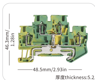
JHST-2.5TBPE
