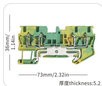
JHST-2.5QWPE
