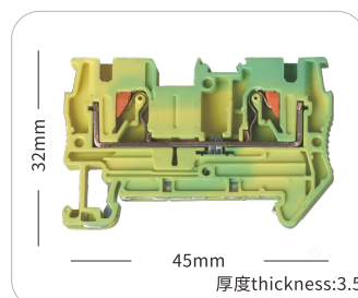
JHPT-1.5PE
