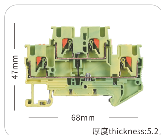
JHPT-TBPE
