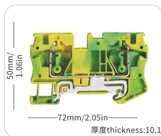
JHST-10PE
