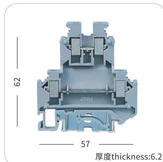
JHUKK 5
