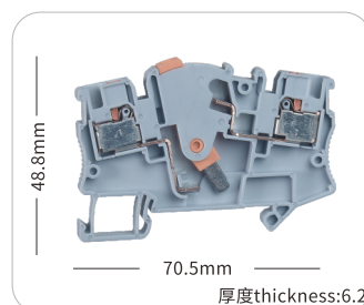
JHPTV-4ME
