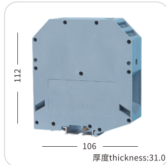
JHUK150
