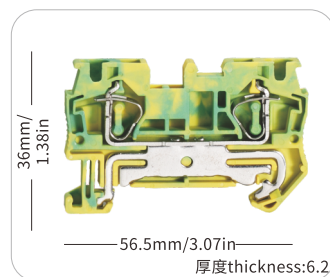
JHST-4PE
