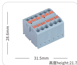
JHPTX-12
